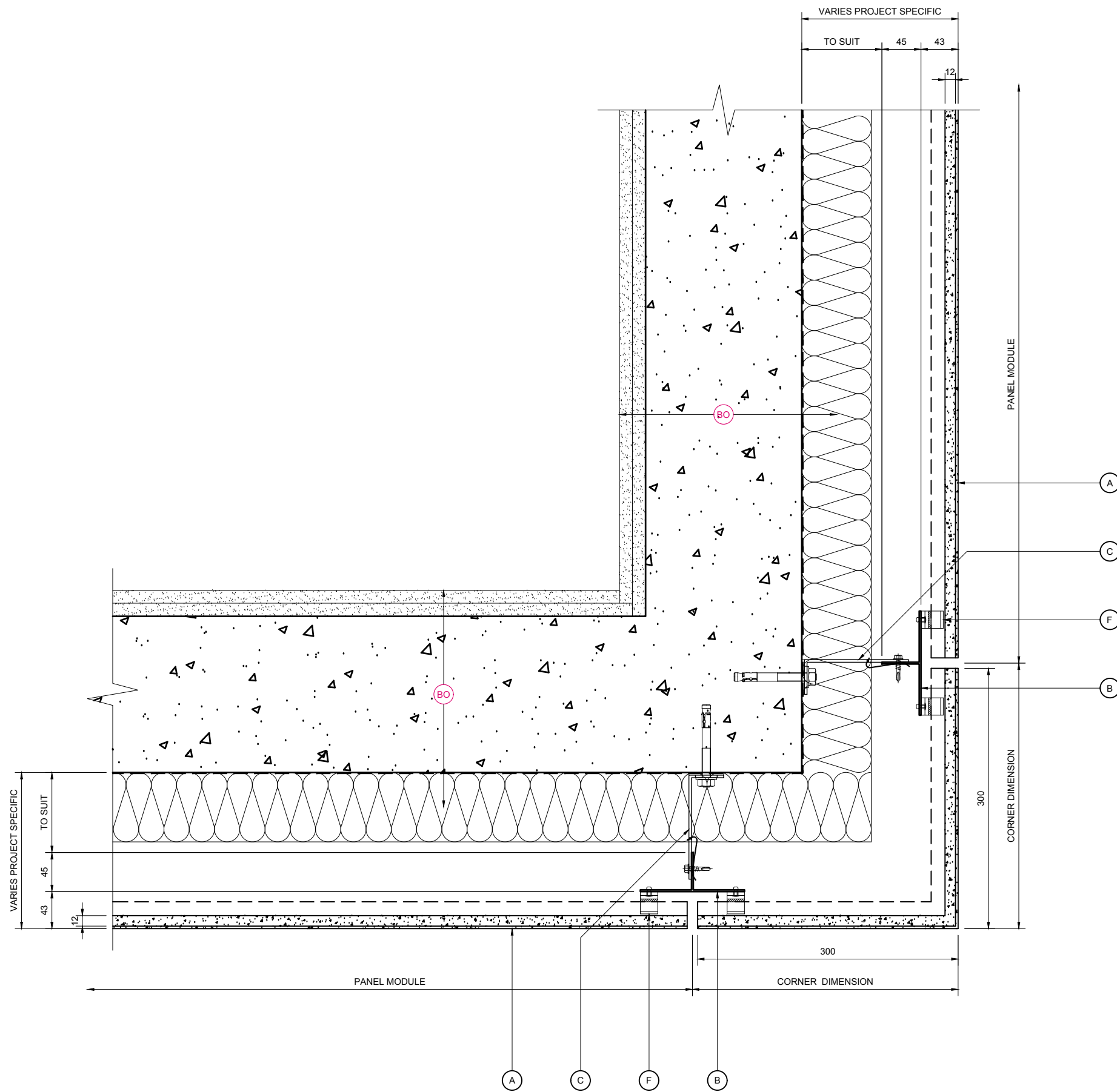
EXTERNAL CORNER PANEL DETAIL
