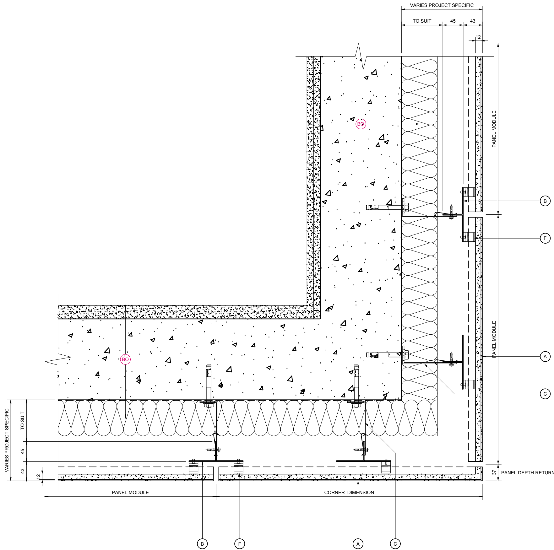
EXTERNAL CORNER DETAIL
